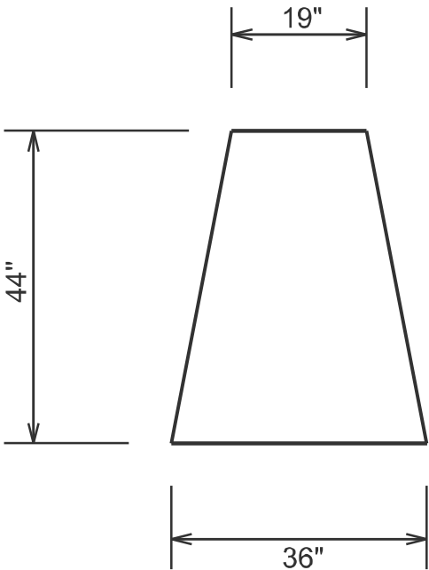
TRANSITION FROM NORMAL CROSS-SECTION
