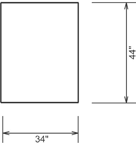
TRANSITION TO MATCH THE CROSS-SECTION OF THE PROPOSED BRIDGE PIERS
