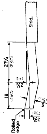
SECTION B-B
