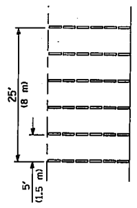
TYPICAL INSTALLATION
