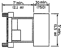
TYPE B ROOF OR TRAILER MOUNTED ARROW BOARDS
