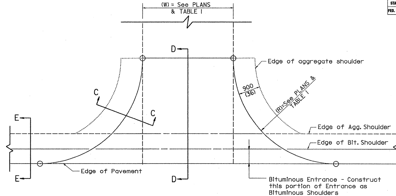
PLAN PCC OR BITUMINOUS ENTRANCE
