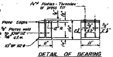
DETAIL OF BEARING AT PIER 4
