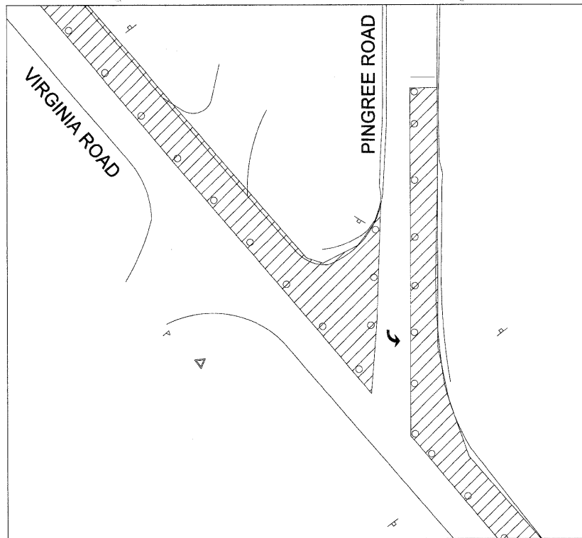
PINGREE ROAD MOT STAGE IIA DETAIL
