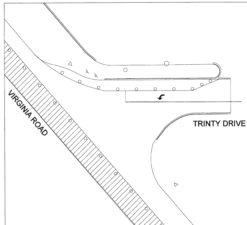
TRINITY DRIVE MOT STAGE I DETAIL
