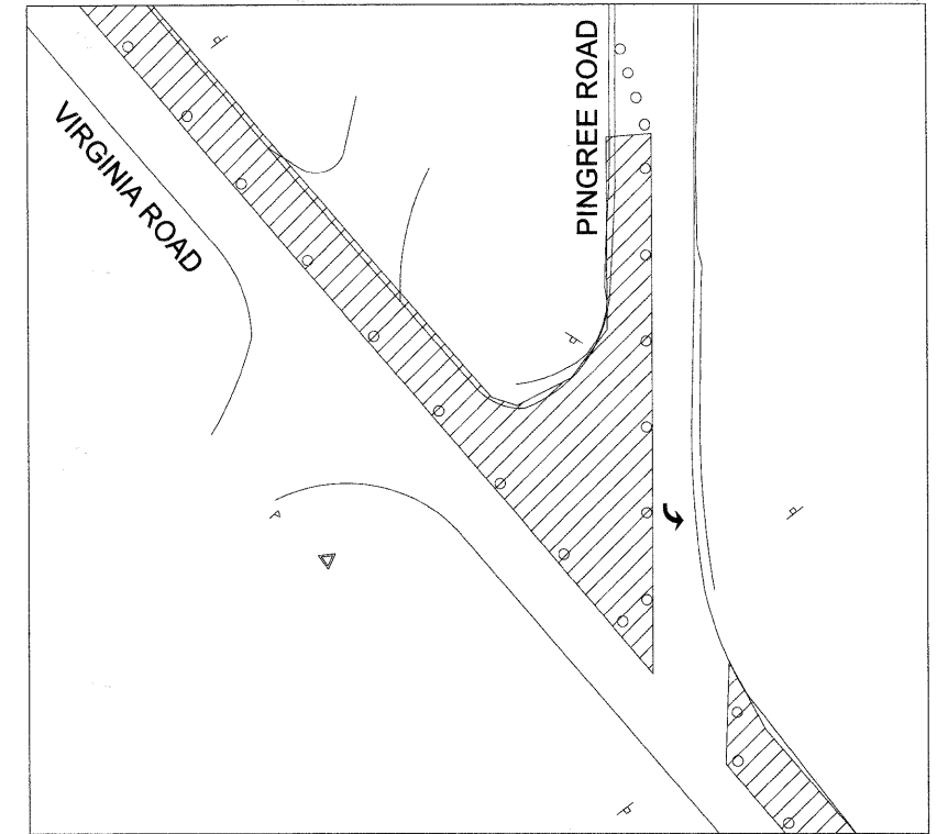
PINGREE ROAD MOT STAGE IIB DETAIL
