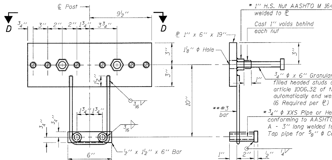
ANCHOR DEVICE
