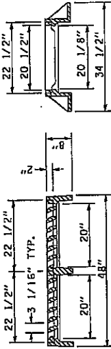
NEENAH FRAME AND GRATE NO. R-3527-M
