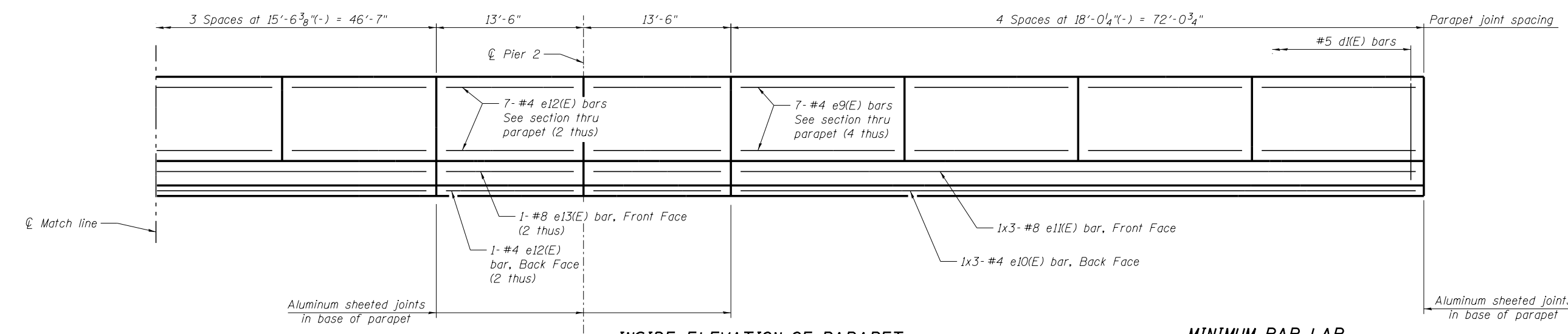
INSIDE ELEVATION OF PARAPET (West parapet shown, east parapet similar)
