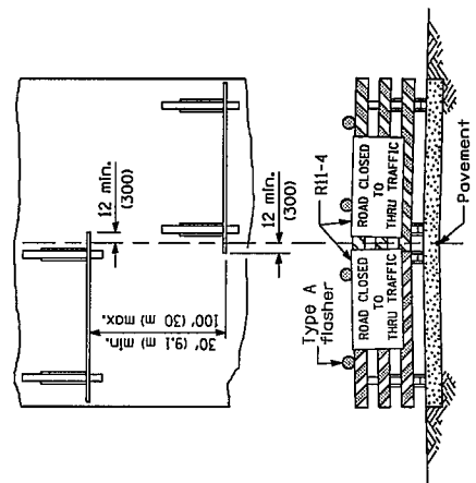
ROAD CLOSED TO THRU TRAFFIC ReflectORIZED striping shall appear on both sides of the barricades. If a Type III barricade with an attached sign panel which meets NCHRP 350 is not available, the signs may be mounted on NCHRP 350 temporary sign supports directly in front of the barricade.
