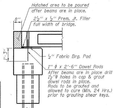
SECTION AT ABUTMENTS
