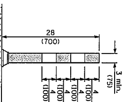
FLEXIBLE DELINEATOR
