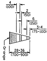
ORANGE REFLECTORIZED CONE
