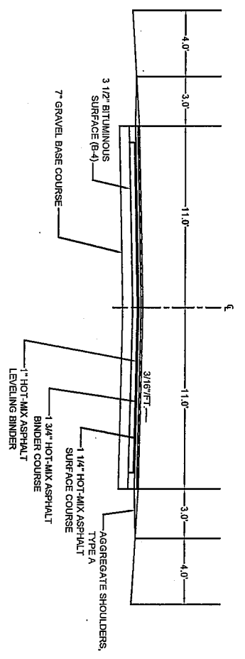
EXISTING TYPICAL SECTION FROM SEC. 83-00147-00-RS STA. 524+00 TO STA. 539+48.20
