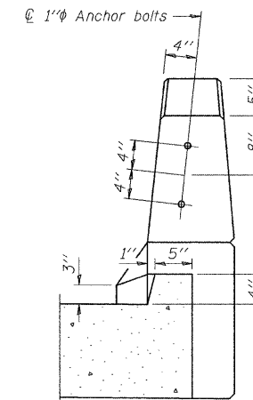
VIEW B-B
