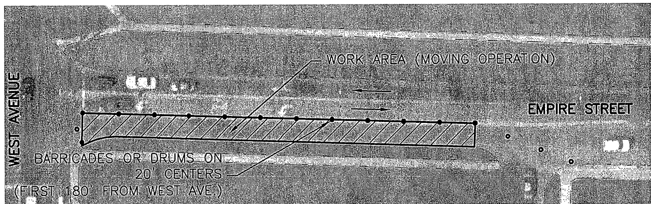
SOUTH LANE CLOSURE – EMPIRE STREET
