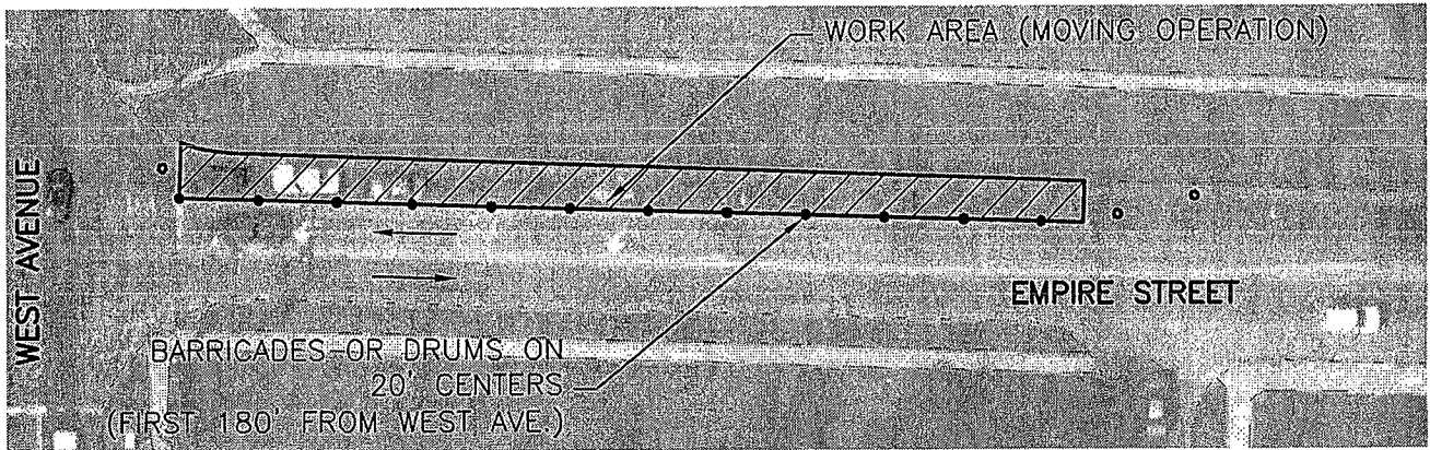
NORTH LANE CLOSURE – EMPIRE STREET
