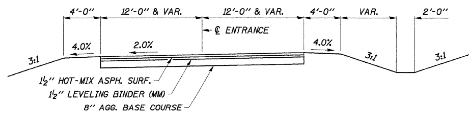
SECTION B-B
