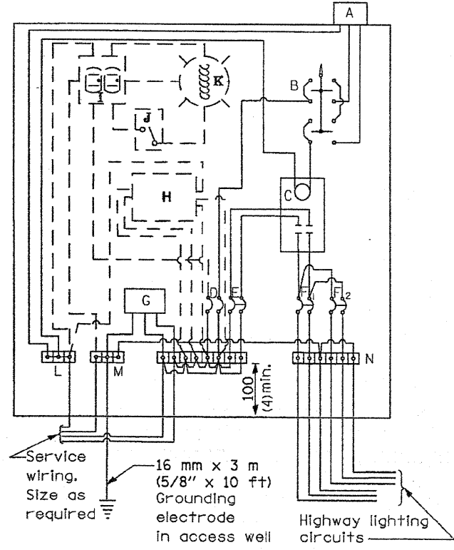
CONTROL SCHEMATIC
