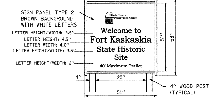
ALL TIMBER POSTS AND FRAMES SHALL BE TREATED IN ACCORDANCE WITH SECTION 1007 OF THE STANDARD SPECIFICATIONS.
