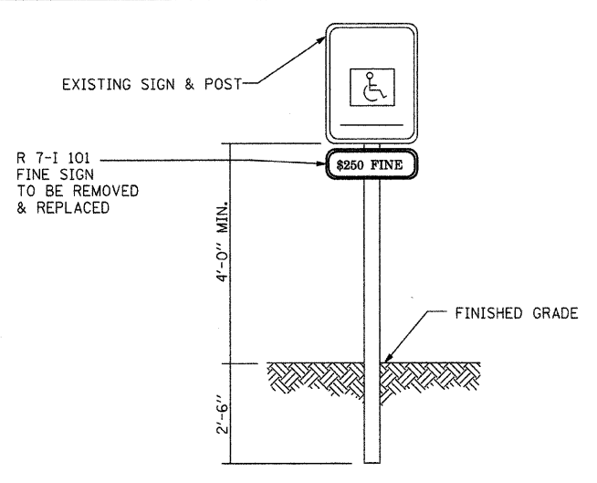
HANDICAPPED PARKING SIGNS NOT TO SCALE
