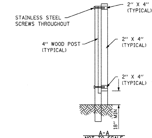
ALL TIMBER POSTS AND FRAMES SHALL BE TREATED IN ACCORDANCE WITH SECTION 1007 OF THE STANDARD SPECIFICATIONS.
