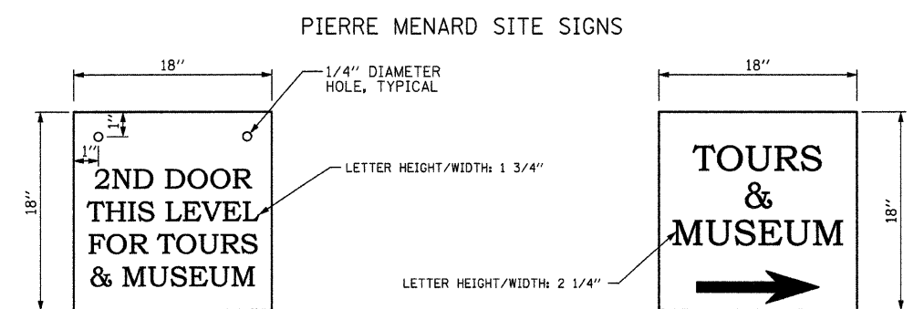
PIERRE MENARD HOME SIGN NOT TO SCALE
