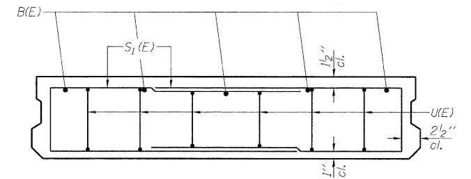
VIEW B-B
