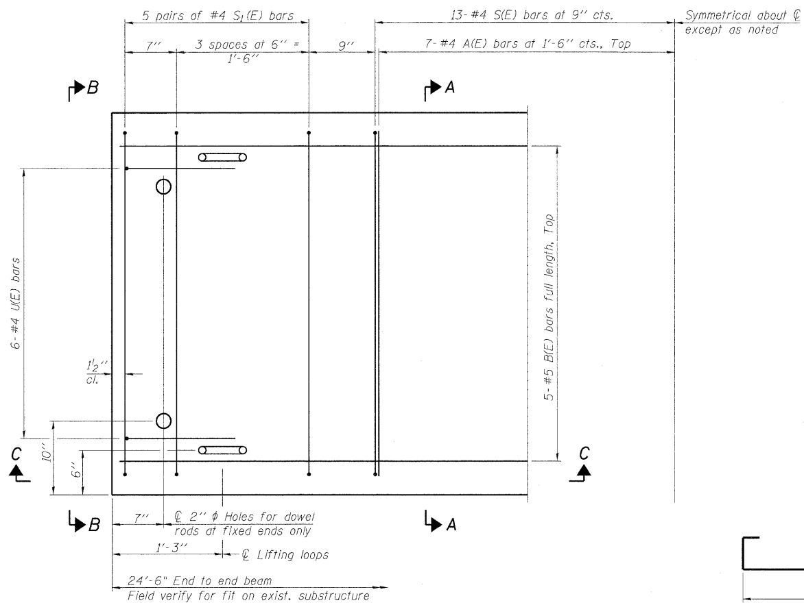
PLAN VIEW
