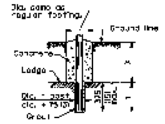
FOOTING FOR POST IN ROCK LEDGE
