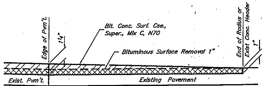
SECTION A-A SIDE ROAD (Est. No. = 20) STATION 0+01 - STATION 51+95
