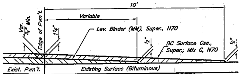
SECTION A-A PRIVATE ENTRANCE - BITUMINOUS (Est. No. = 8)
