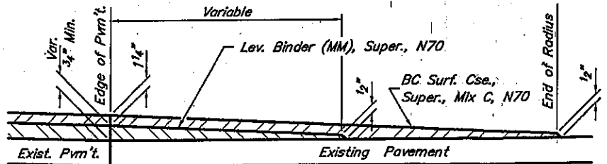
SECTION A-A SIDE ROAD (Est. No. = 4) STATION 70+05 - STATION 192+00
