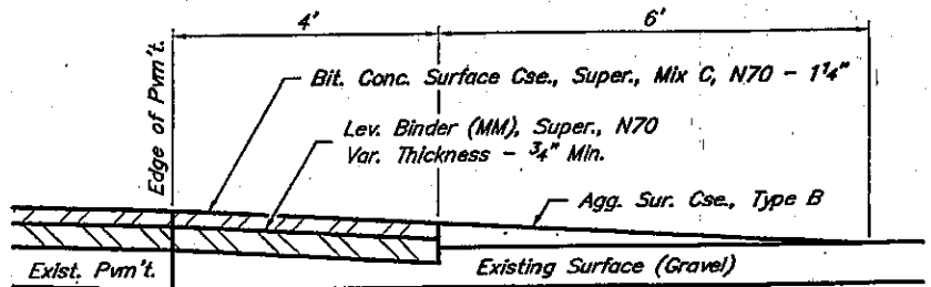
SECTION A-A PRIVATE ENTRANCE - GRAVEL (Est. No. = 16)
