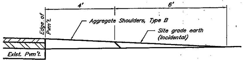
SECTION A-A FIELD ENTRANCE (Est. No. = 2)
