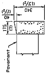
DEPRESSED CURB
