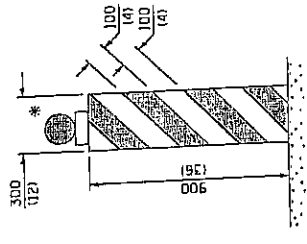
VERTICAL BARRICADE
