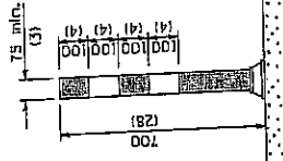
FLEXIBLE DELINEATOR
