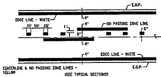
PAVEMENT MARKING
