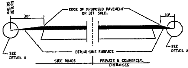
SECTION A-A DETAILS AT ENTRANCES & SIDE ROADS
