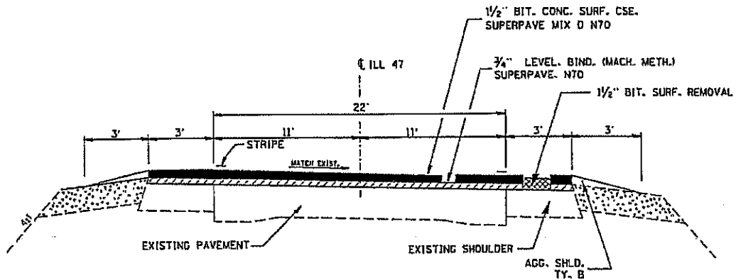
TYPICAL SECTION BEGIN REMOVAL OF S.E. STA. 100+24.78 ATTAIN NORMAL CROWN STA. 102+64.78 NOTE: BEGIN ATTAINING S.E. STA. 130+98.38 ATTAIN FULL S.E. STA. 133+38.38 BEGIN REMOVAL OF S.E. STA. 164+70.54 ATTAIN NORMAL CROWN STA. 167+10.54 STA. 130+98.38 TO STA. 167+10.54
