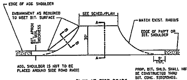
PLAN AT SIDE ROADS
