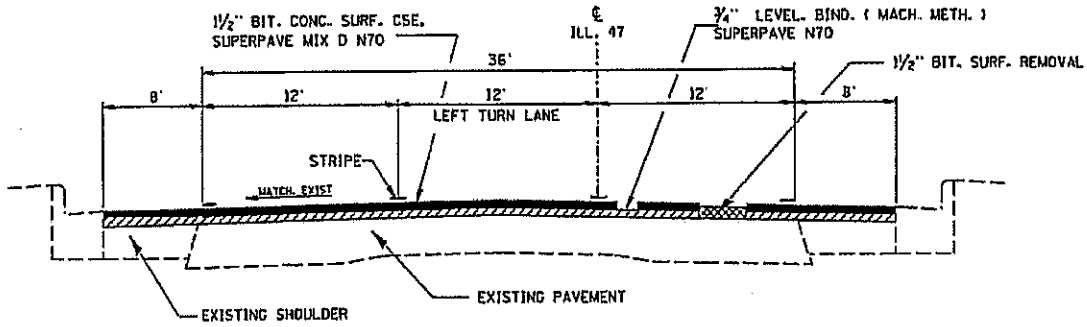
TYPICAL SECTION ILL. 47 - FROM ILL. 47/ILL. 71 INTERSECTION TO STA. 100+60
