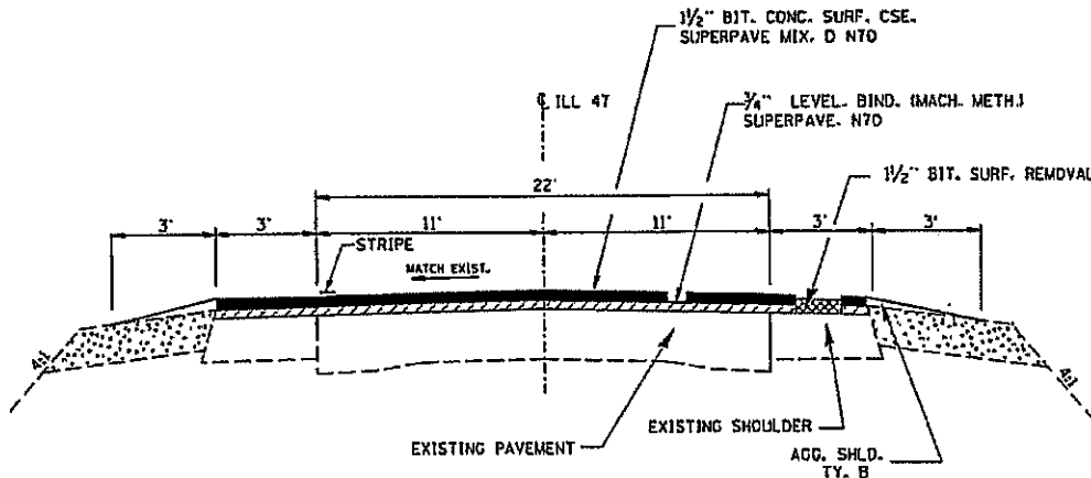
TYPICAL SECTION STA. 100+60 TO STA. 497+50
