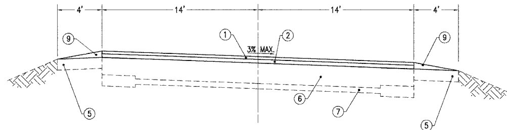
W/SUPERELEVATION - STA. 59+93 TO 64+66
