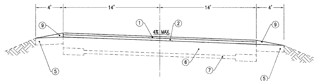
W/SUPERELEVATION - STA. 77+76 TO 83+19
