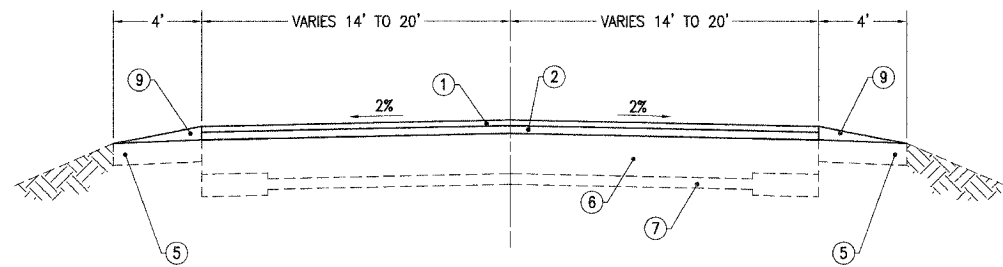
W/O SUPERELEVATION
