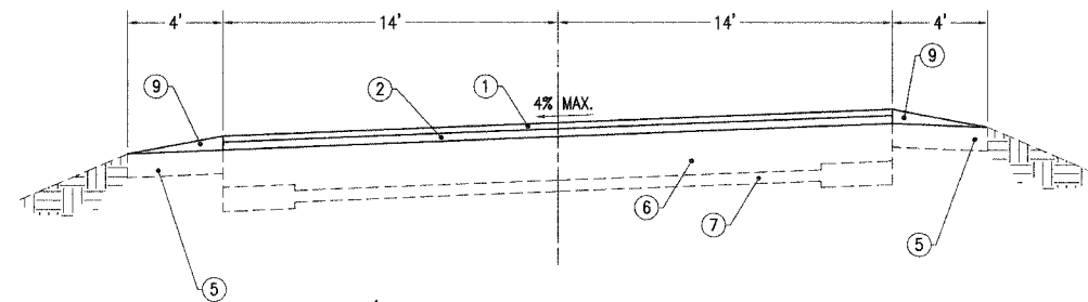
W/SUPERELEVATION - STA. 65+39 TO 73+35
