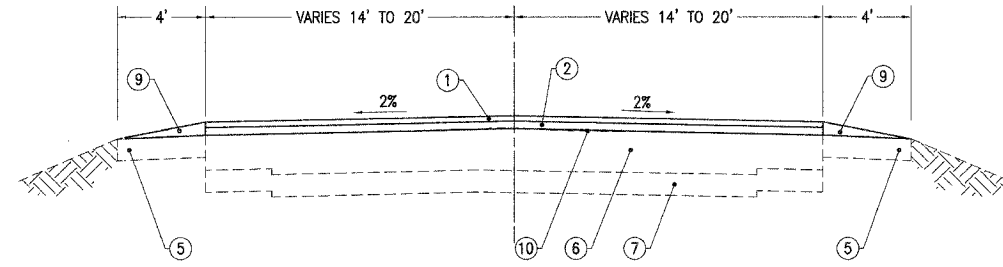
TYPICAL SECTION - STA. 83+00 TO 90+25
