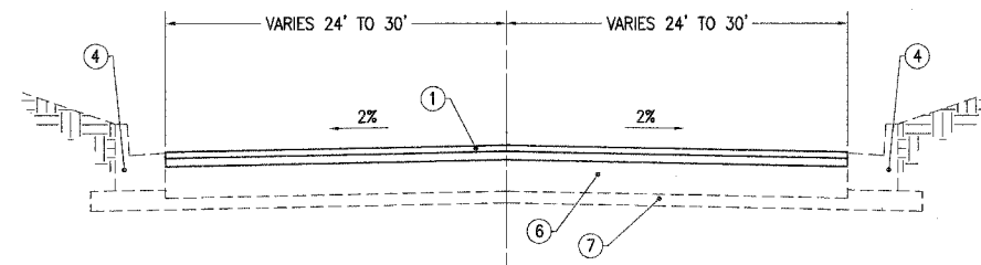
TYPICAL SECTION - STA. 94+95 TO 99+33
