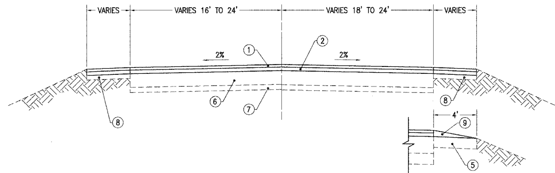
TYPICAL SECTION - STA. 90+25 TO 94+95
