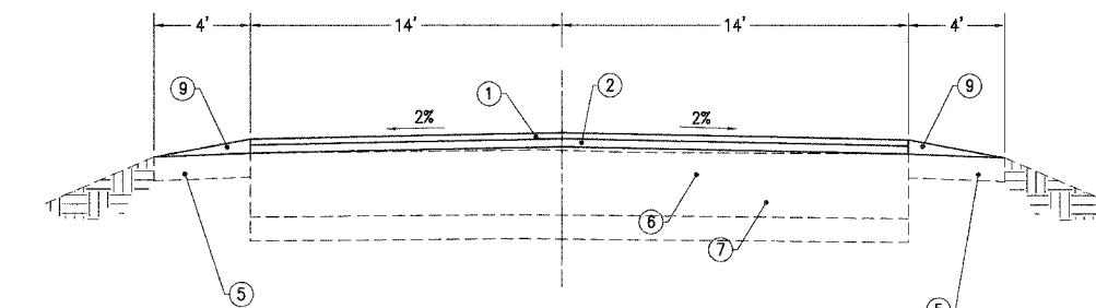
W/O SUPERELEVATION
