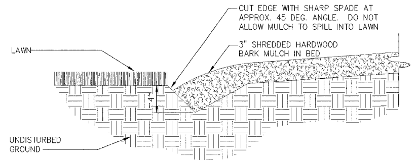
SPADE EDGING DETAIL
