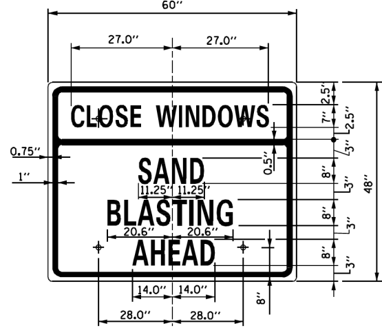
SIGN TS-10 (O)
