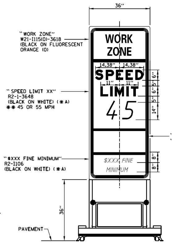
WORK ZONE SPEED LIMIT SIGN ASSEMBLY
