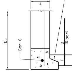
ALTERNATE JOINT CONFIGURATIONS
