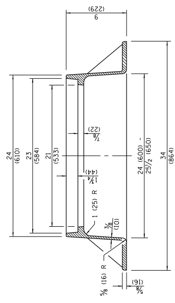
SECTION A-A Gray Iron
