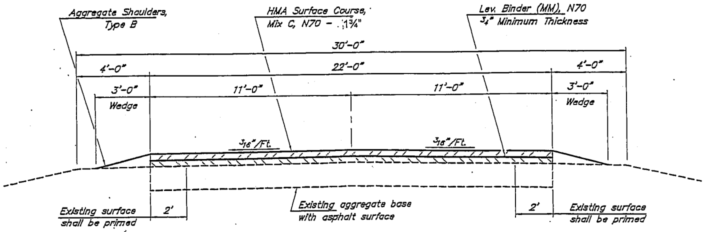
TYPICAL SECTION
