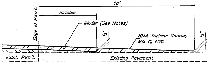
SECTION A-A PRIVATE ENTRANCE - ASPHALT
