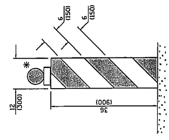
VERTICAL BARRICADE
