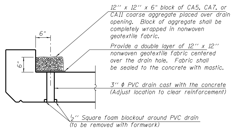
DRAIN DETAIL
