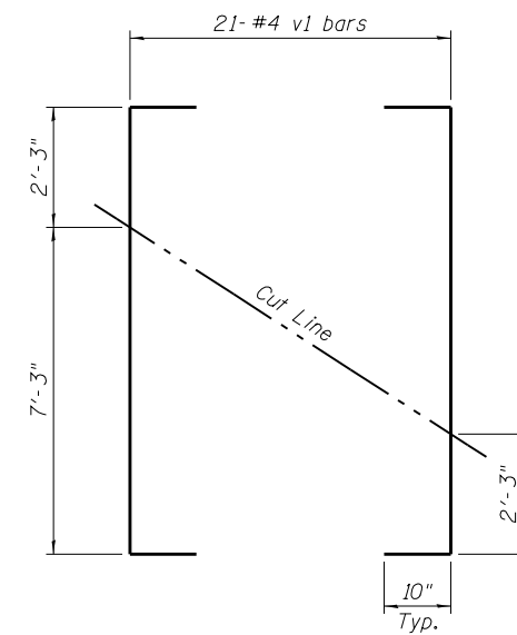
CUTTING DIAGRAM
