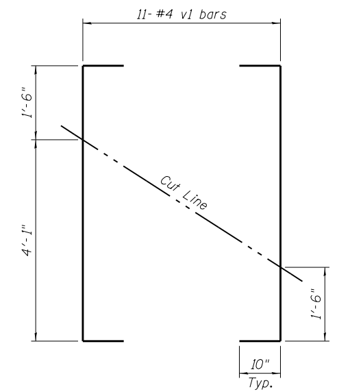
CUTTING DIAGRAM
