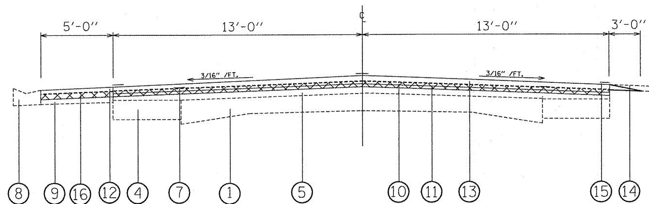
TYPICAL SECTION NO. 5 STA. 107+00 TO STA. 109+60
