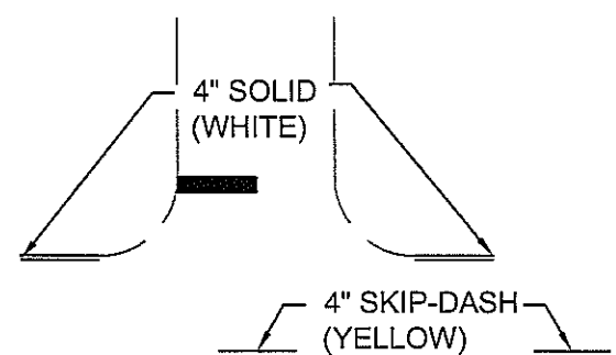
MAIN STREET (MS 2600) NO MAINLINE STOP OPTION
