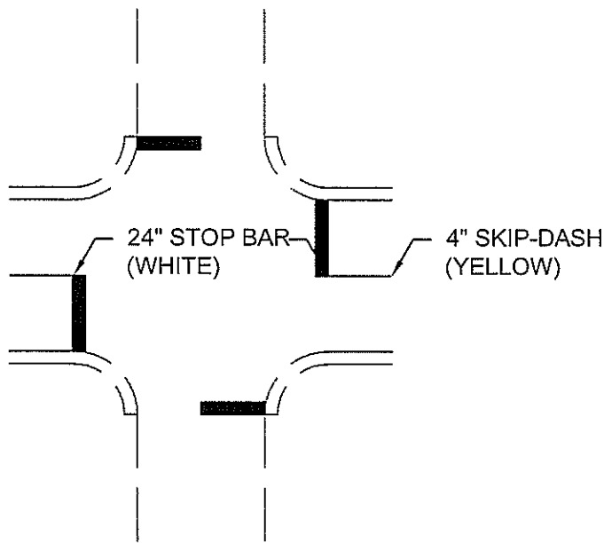
FRANKLIN STREET (MS 2500) 3 OR 4 WAY STOP OPTION
