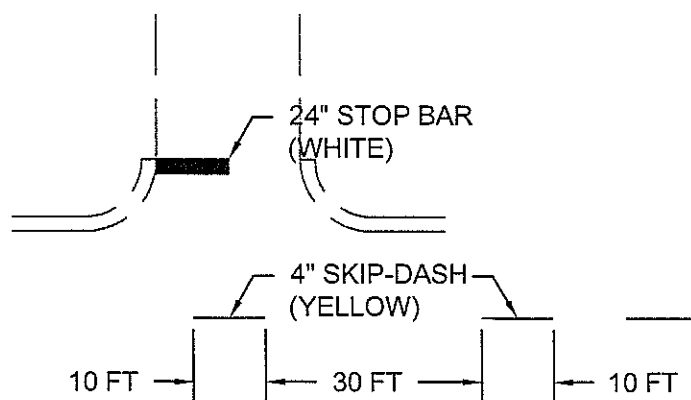
FRANKLIN STREET (MS 2500) NO MAINLINE STOP OPTION
