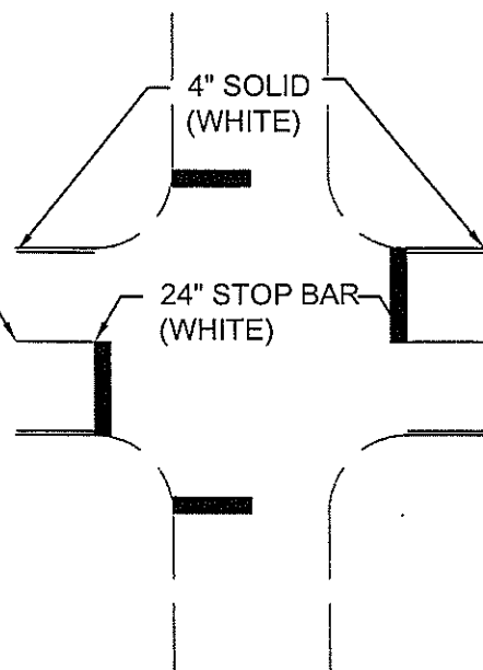
MAIN STREET (MS 2600) 3 OR 4 WAY STOP OPTION
