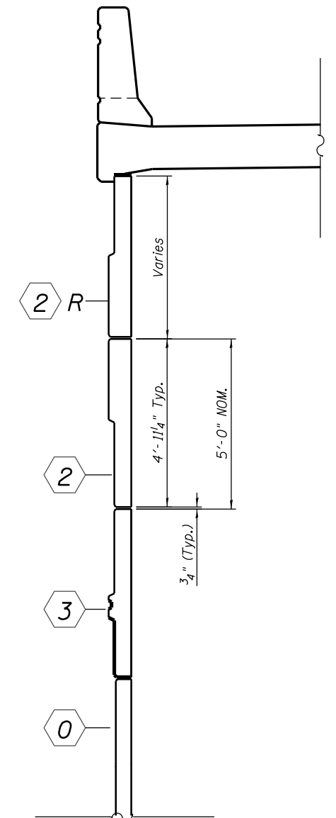
SECTION G-G
