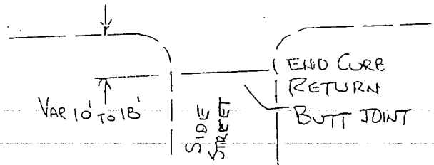
SIDE STREETS PAVE TO END OF CURB RETURN
