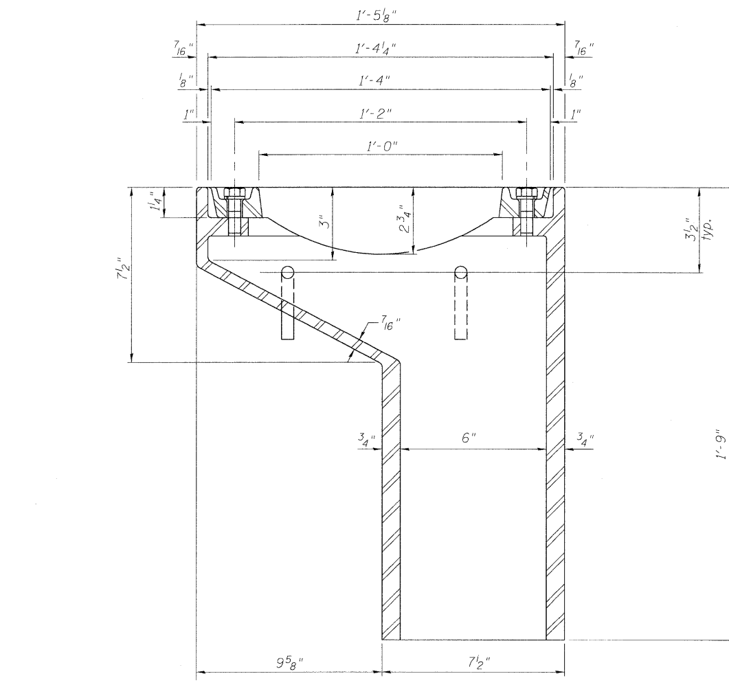
SECTION A-A See sheet 3 of 7 for scupper location relative to parapet.
