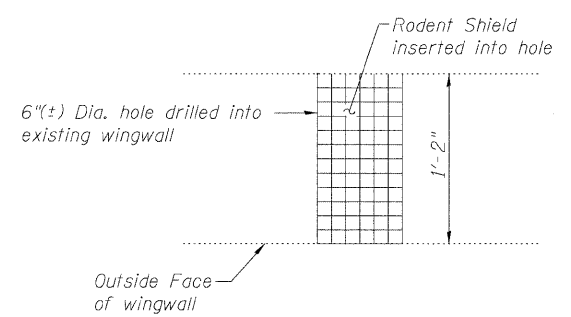
RODENT SHIELD PLACEMENT
