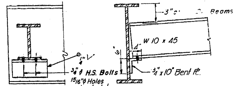
DIAPHRAGM D
