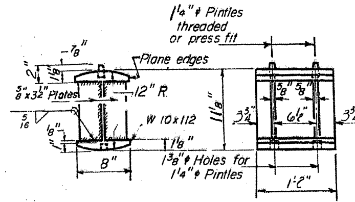
ROCKER
