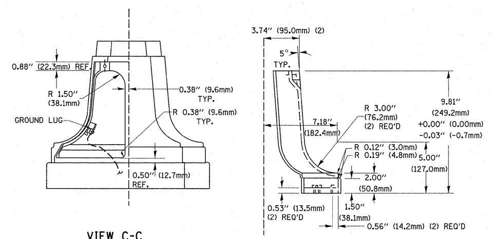
VIEW C-C
