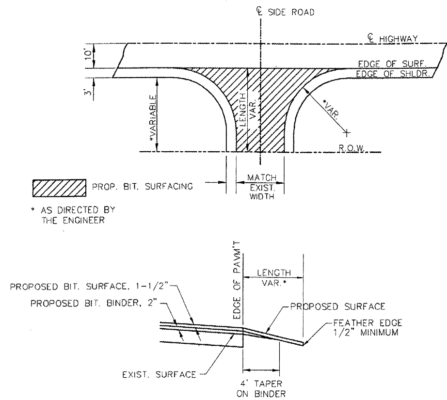
SIDEROAD DETAILS
