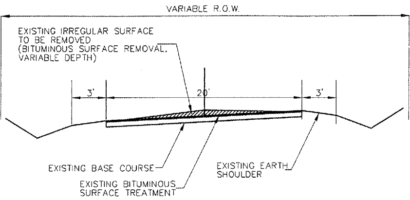
TYPICAL EXISTING SUPERELEVATED SECTION
