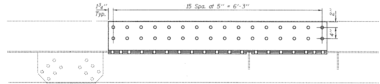
VIEW D-D REPAIR A11 (1 Required)
