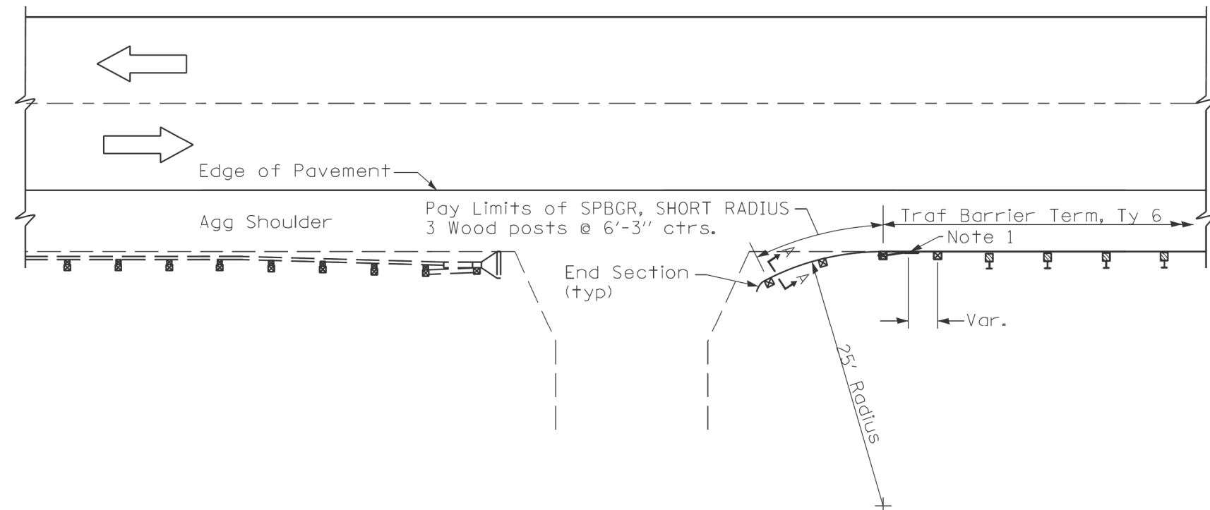
PLAN
