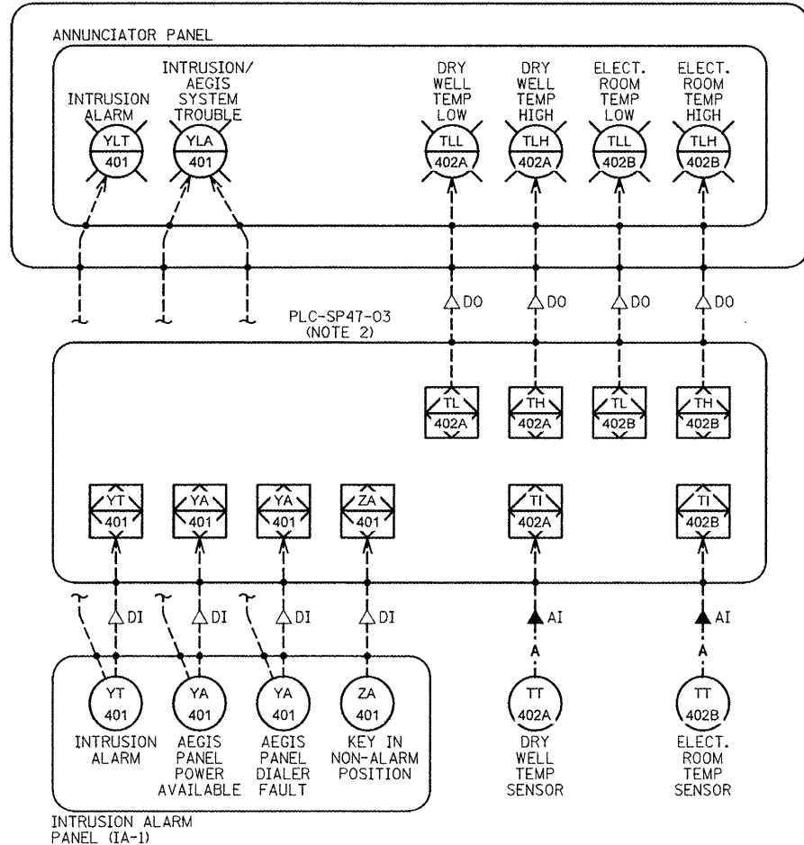
3 GENERAL BUILDING P&amp;ID
