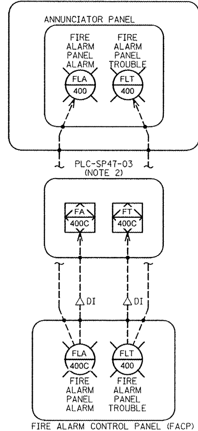
5 FIRE ALARM CONTROL PANEL (FACP) P&amp;ID
