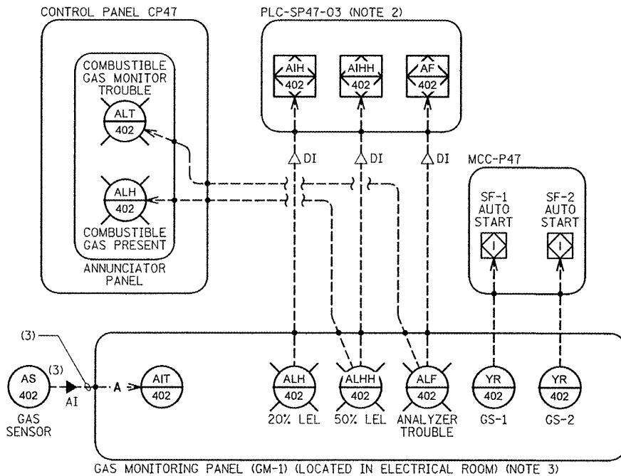
2 GAS MONITORING PANEL P&amp;ID
