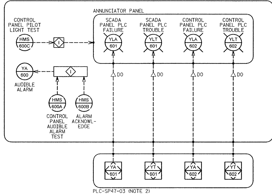
1 MISCELLANEOUS CONTROL PANEL P&amp;ID
