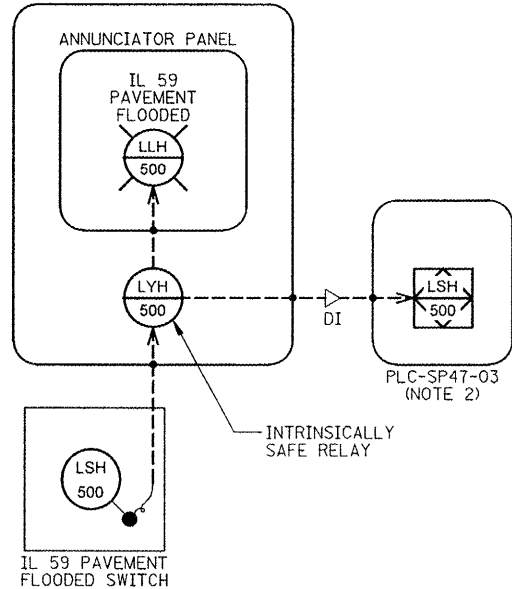
4 PAVEMENT FLOOD SYSTEM P&amp;ID
