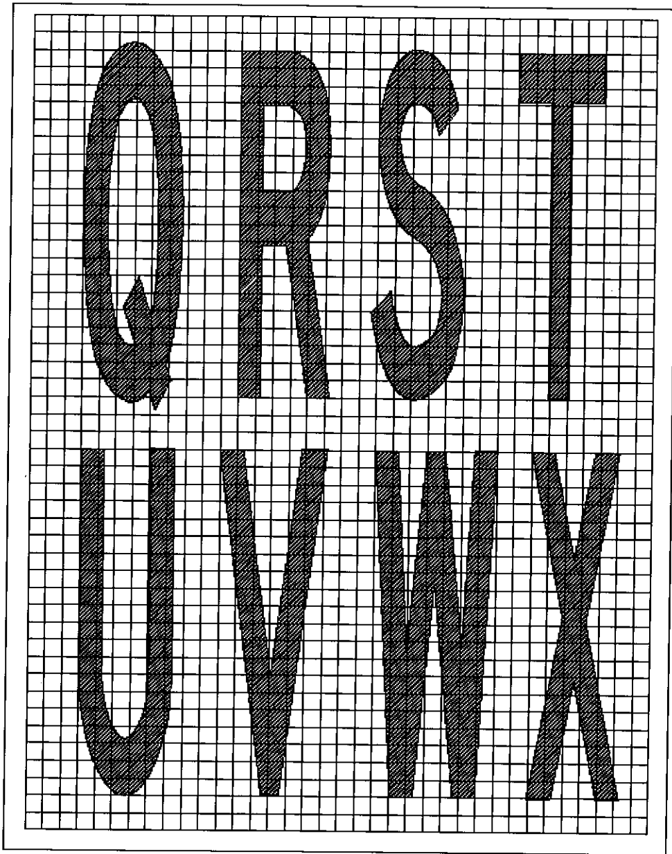
Figure A-3. Pavement Markings QRSTUVWX
