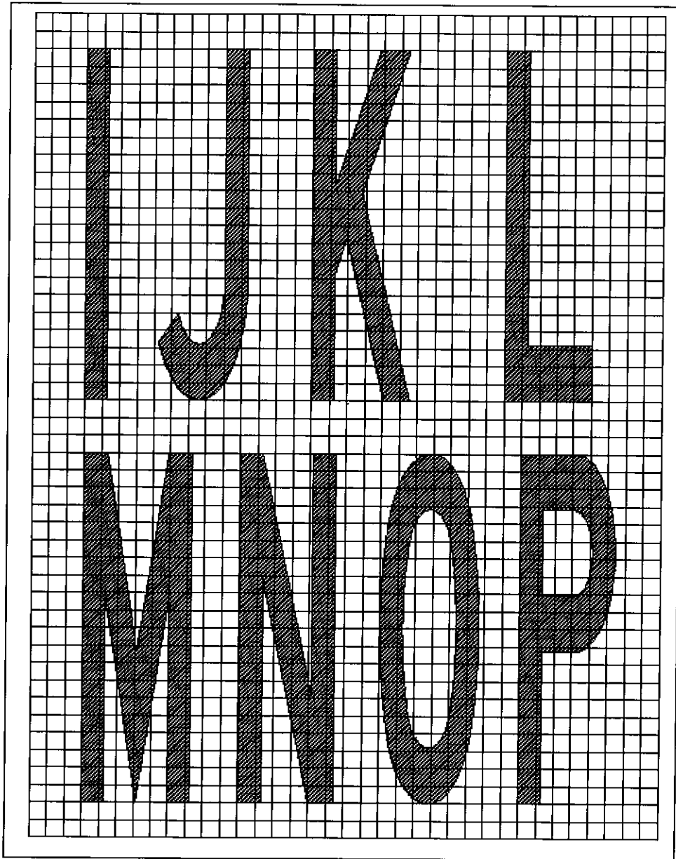
Figure A-2. Pavement Markings IJKLMNOP
