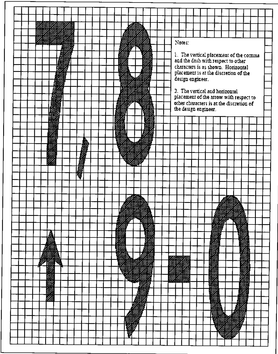
Figure A-5. Pavement Markings 7890-↑
