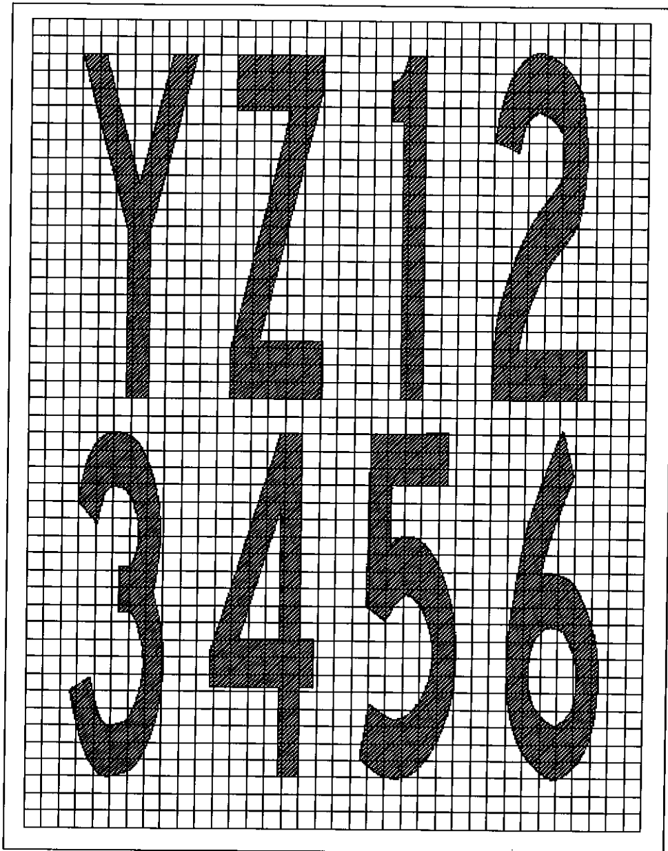
Figure A-4. Pavement Markings YZ123456
