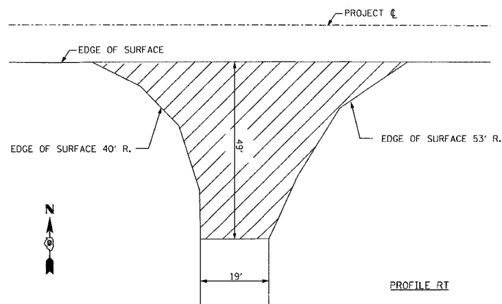
DETAIL OF INTERSECTION RT. STA. 43+33
