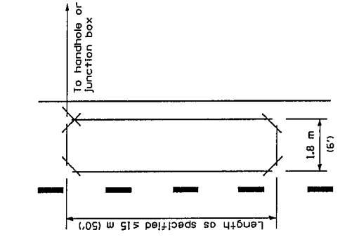
FOR PRESENCE DETECTION LONG LOOP
