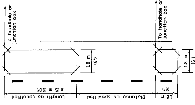
FOR EXTENDED-CALL DETECTION
