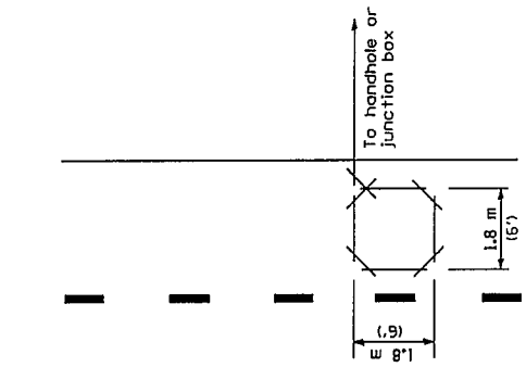
FOR POINT DETECTION SHORT LOOP
