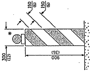
VERTICAL BARRICADE
