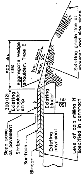
COLD MILLING AND/OR RESURFACING OF EXISTING PAVEMENT WITH SHOULDER STRIPS (Cross-section D)
