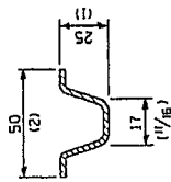
SECTION E-E
