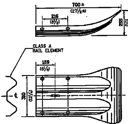
END SECTION
