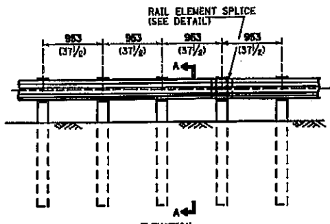
ELEVATION TYPE B 963 (37 1/2") CLOSED POST SPACING
