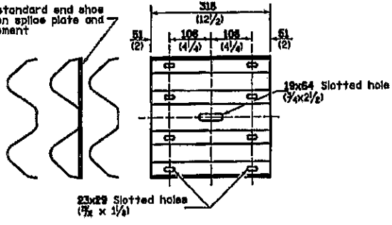
SPLICE PLATE
