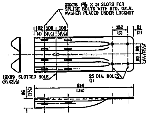
END SECTION
