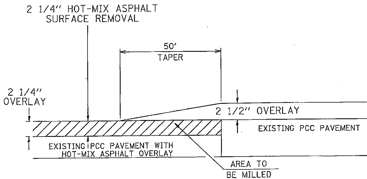
TAPER DETAIL @ EILER ROAD (EAST & WEST) (NTS)
