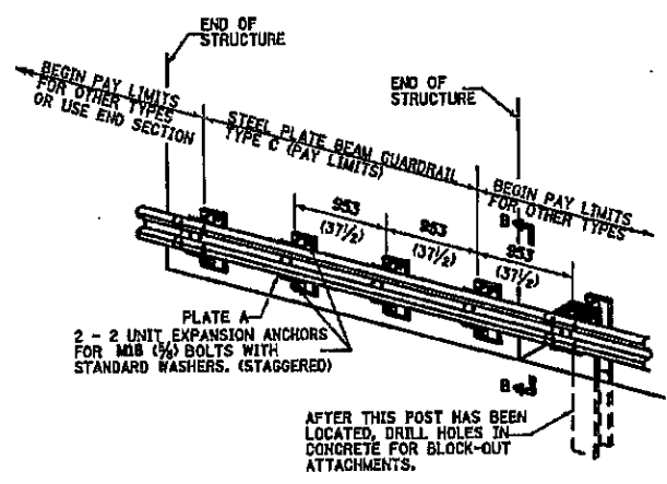
TYPE C 963 (37 1/2") BLOCK-OUT SPACING
