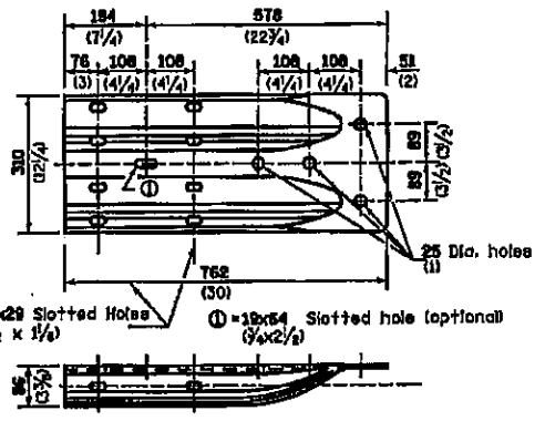
ALTERNATE END SHOE
