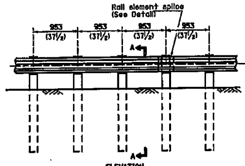
ELEVATION TYPE B
