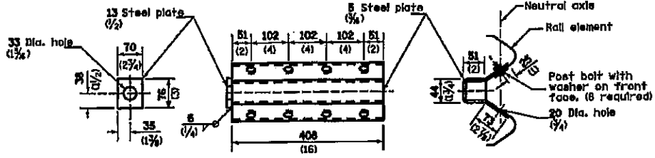
ANCHOR PLATE T DETAILS
