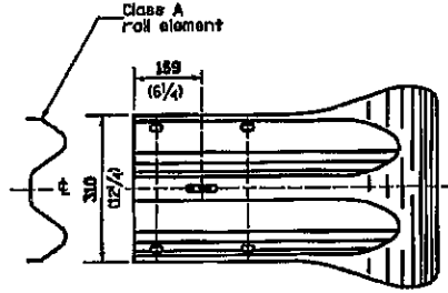
END SECTION
