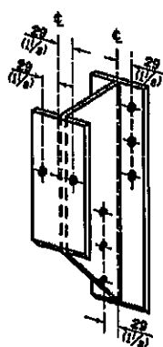
STEEL BLOCK-OUT DETAIL
