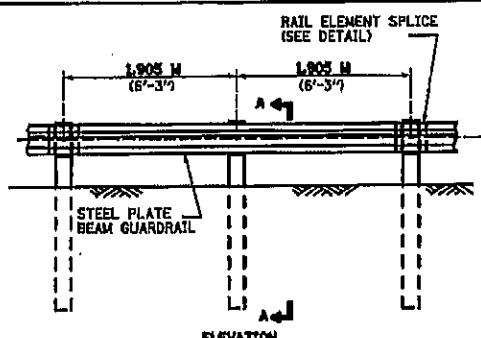
ELEVATION TYPE A 1.905 M (6'-3 1/4") TYPICAL POST SPACING
