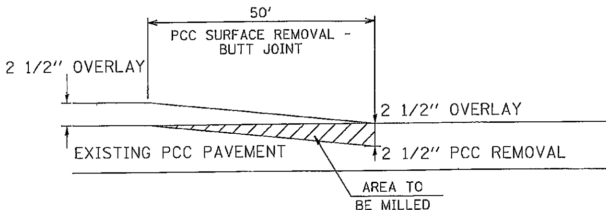
PCC BUTT JOINT DETAIL @ EILER ROAD (SOUTH) (NTS)
