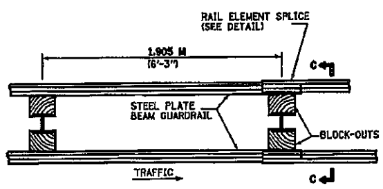
PLAN TYPE D DOUBLE STEEL PLATE BEAM GUARDRAIL 1.905 M (6'-3 1/4") TYPICAL POST SPACING
