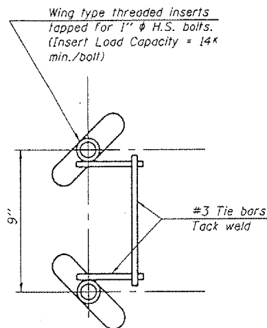
INSERT DETAIL
