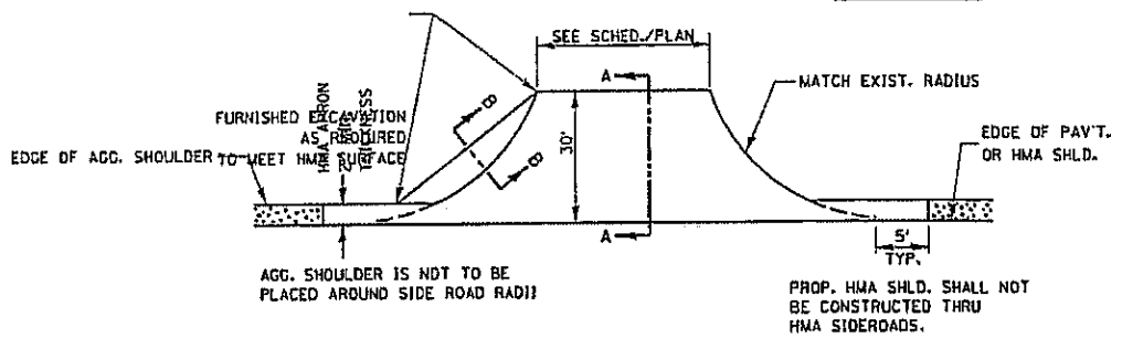
PLAN AT SIDE ROADS
