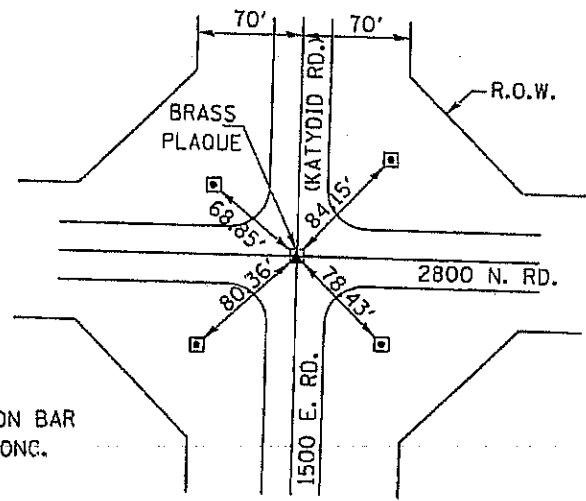
N.E. CORNER SECTION 33 T. 30 N., R. 5 E. 3rd P.M. LIVINGSTON COUNTY
