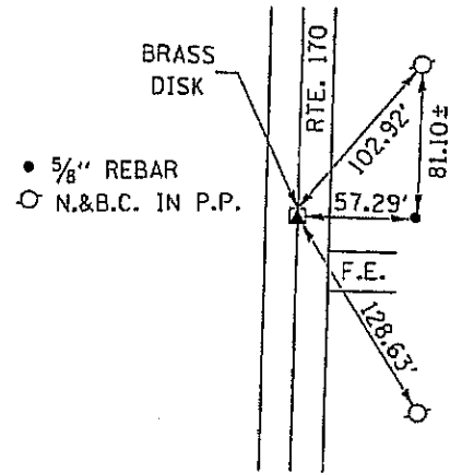
E. 1/4 CORNER SECTION 21 T. 30 N., R. 5 E. 3rd P.M. LIVINGSTON COUNTY
