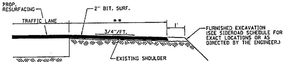
SECTION A-A MAILBOX TURNOUT DETAILS
