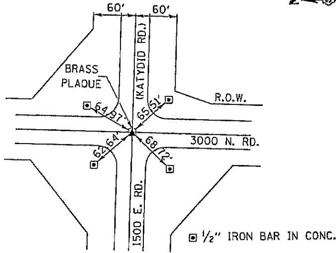
N.E. CORNER SECTION 21 T. 30 N., R. 5 E. 3rd P.M. LIVINGSTON COUNTY
