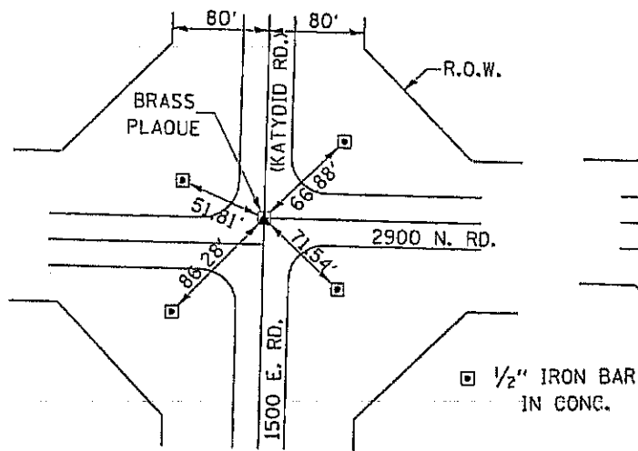
S.E. CORNER SECTION 21 T. 30 N., R. 5 E. 3rd P.M. LIVINGSTON COUNTY
