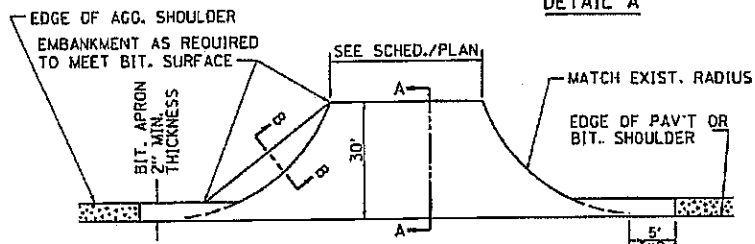
DETAIL A
